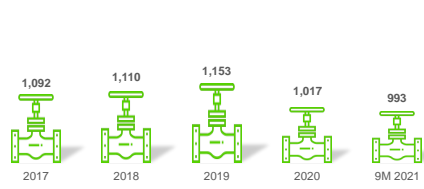
Transported Volumes (mboed) 2017 - 9M 2021
